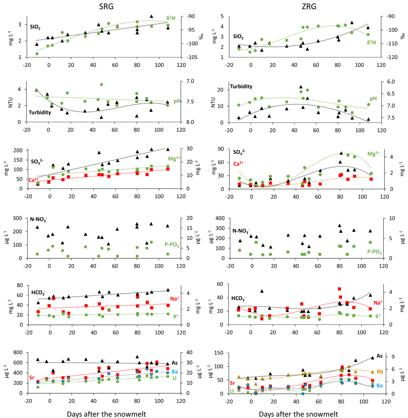
FIGURE 4 Seasonal trends of water parameters over summer, as a function of the days after the snowmelt end (reference Madriccio station, APB, 2020a) at SRG (left panels) and ZRG (right panels). In each scatterplot, distinct parameters are shown in different colours and shapes, and their scale corresponds to that of the axis where the name of each parameter is placed. Interpolation lines represent linear regression or polynomial smoothing curves of level three (turbidity at SRG, smoothing curves for ZRG)
