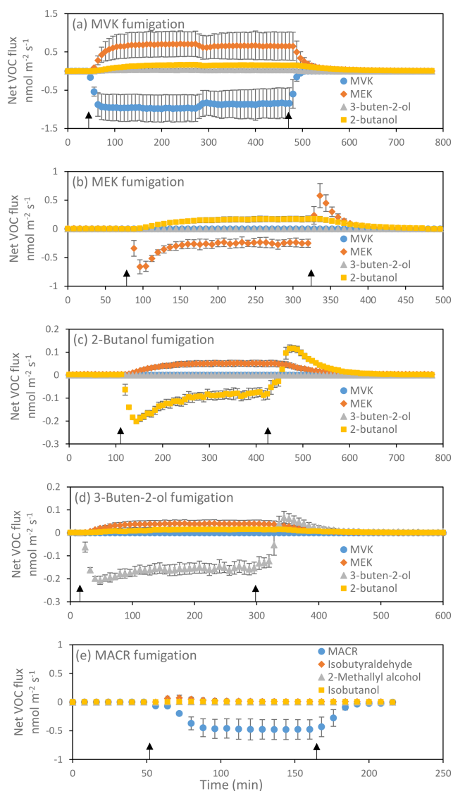
Figure 1. Uptake of MVK (a), MEK (b), 2-butanol (c), 3-buten-2-ol (d) and MACR (e) and emission of their oxidized or reduced products in red oak leaves. Results are reported as mean \pm standard deviation ( n = 3 ). Negative values denote the uptake and positive values the emission of volatiles. Black arrows indicate the beginning and the end of the fumigation. In (b), the pulses of MEK uptake at the beginning of the fumigation and of MEK release after the end of the fumigation correspond to formation and release, respectively, of a MEK pool dissolved into the leaf water. At equilibrium the uptake of MEK and subsequent release of 2-butanol is constant and indicates a constant rate of MEK transformation within leaves. Analogous considerations can be made for 2-butanol and 3-buten-2-ol in (c) and (d), respectively.
