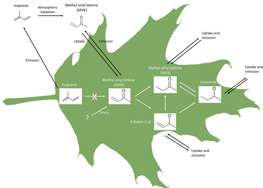
Figure 5. Schematics of MVK, MEK, 3-buten-2-ol, and 2-butanol origin and interconversion in leaves, as suggested by this study. The uptake of MEK, 3-buten-2-ol, and 2-butanol has not been reported so far but it is in principle possible given the present results.
