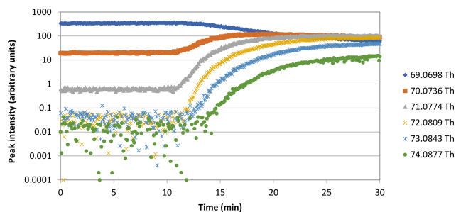
Figure 3. Labelling of isoprene emitted by red oak leaves upon ^{13}\text{CO}_2 -feeding in the air. Fully labelled ^{13}\text{CO}_2 is constantly supplied to the plants starting from time T = 10 min.
