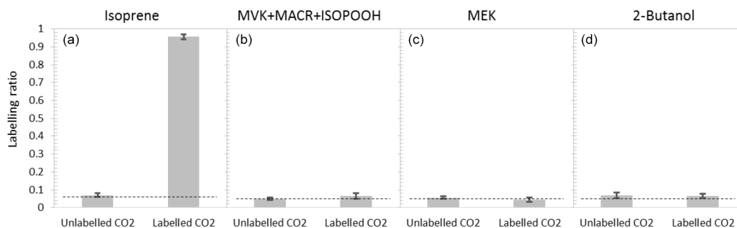
Figure 4. Emission of isoprene (a), MVK + MACR + ISOPOOH (b), MEK (c), and 2-butanol (d) in red oak plants heat stressed at 45 °C for 2 h in the light, under 12 CO 2 or 13 CO 2 atmosphere. Dashed horizontal lines represent natural abundances of isotopic compounds.
