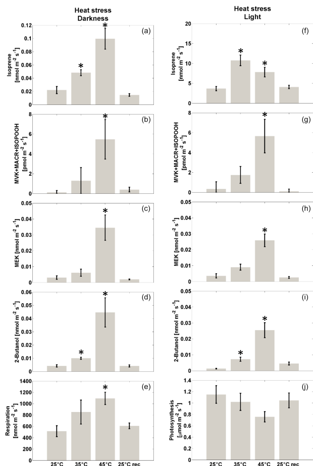
Figure 2. Left: net flux of isoprene (a), MVK + MACR + ISOPOOH (b), products from MVK reduction (MEK, c, and 2-butanol, d) and respiration (e) upon exposure to moderate (35 °C) or severe (45 °C) heat stress, and recovery to 25 °C by red oak plants in the dark. The compound grouping is based on PTR-ToF-MS in \text{H}_3\text{O}^+ mode. Results are reported as mean \pm standard error ( n = 6 ). Asterisks indicate significant differences (Kruskal–Wallis, p < 0.05 ) compared to the unstressed (25 °C) case. Right: emission of isoprene (f), MVK + MACR + ISOPOOH (g), products from MVK reduction (MEK, h, and 2-butanol, i), and photosynthesis (j) upon exposure to moderate (35 °C) or severe (45 °C) heat stress, and recovery to 25 °C in red oak plants in the light (ca. 90 \mu\text{mol m}^{-2} \text{s}^{-1} light intensity). The compound grouping is based on PTR-ToF-MS in \text{H}_3\text{O}^+ mode. Results are reported as mean \pm standard error ( n = 6 ). Asterisks indicate significant differences (Kruskal–Wallis, p < 0.05 ) compared to the unstressed (25 °C) control.
