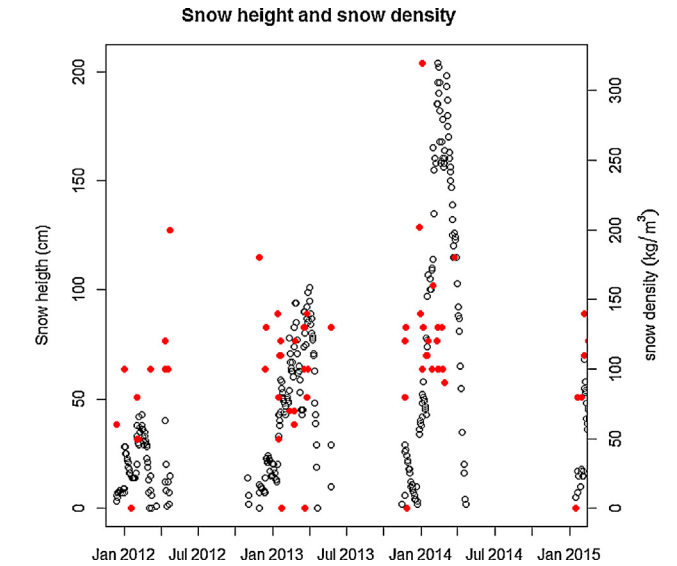
Fig. 5. Measured snow height and snow density during the years 2012, 2013 and 2014. The snow height (cm) is depicted by the black dots and the snow density (kg/m 3 ) by the red points. The values are not measured on site but at nearby a meteorological site.
