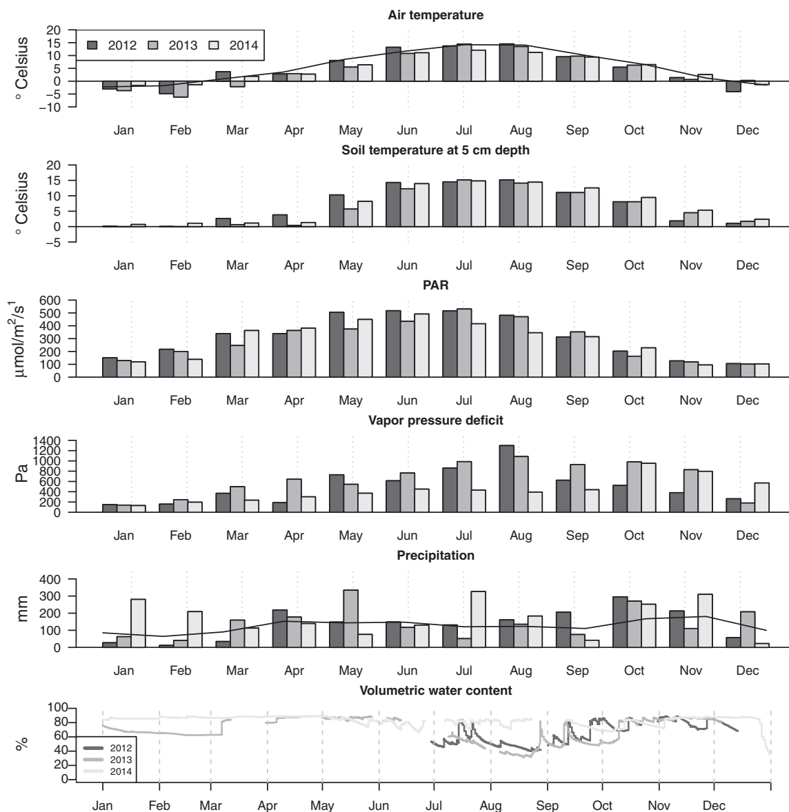
Fig. 3. Monthly values for meteorological variables across 3 years: average air temperature with the long-term average (Eccel et al., 2012) as a solid line, average soil temperature at 5 cm depth, total photosynthetic active radiation (PAR), mean vapour pressure deficit, total precipitation, and volumetric water content under Calluna vulgaris at 5 cm depth.
