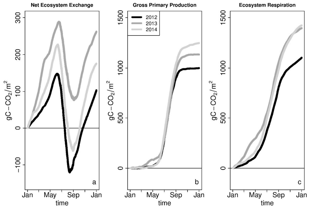
Figure 4-6a Cumulative NEE flux for each year b) Cumulative GPP flux for each year c) Cumulative R_{eco} flux for each year.
