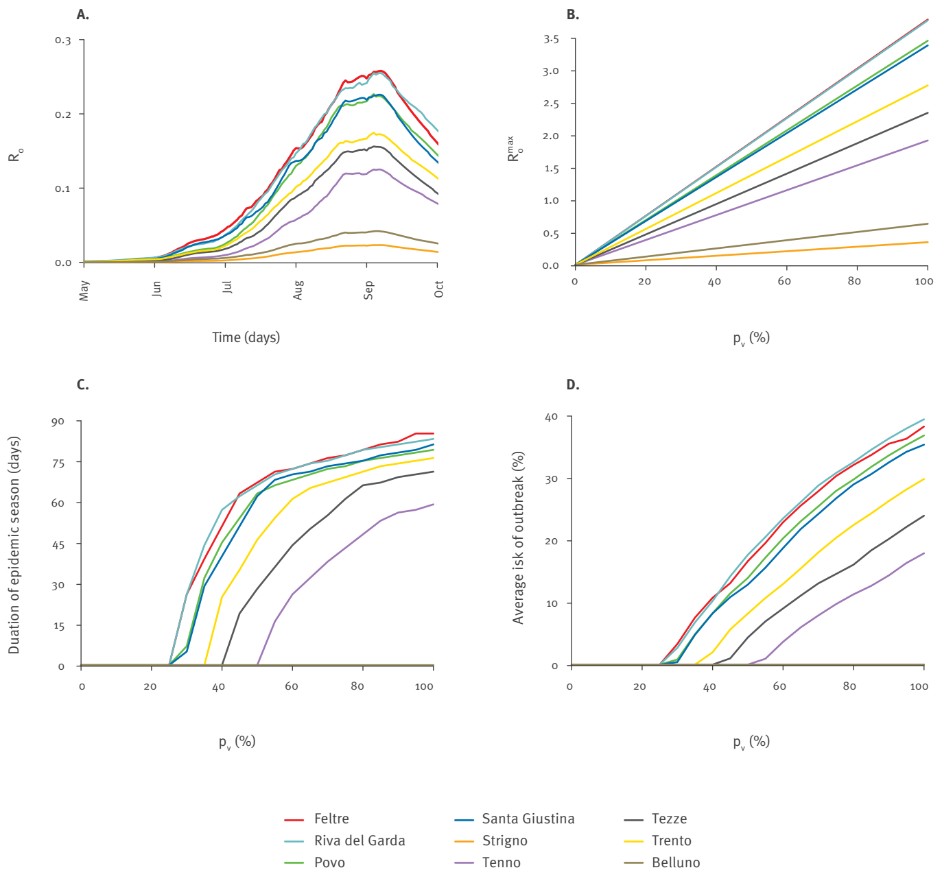
B: Maximum value of R_0 during the year. C: Duration of the epidemic season, defined as the time interval of the year when R_0 > 1 . D: Average risk of outbreaks per imported case over the epidemic season.
