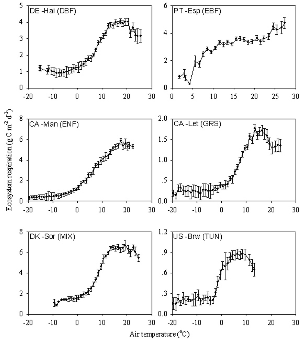
Figure 1. Examples of temperature response curves of ecosystem respiration with standard errors. DBF: deciduous broadleaf forest; EBF: evergreen broadleaf forest; ENF: evergreen needleleaf forest; GRS: grassland; MIX: mixed forest; TUN: tundra. Annual mean temperature at US-Brw and CA-Man are below 0°C.
