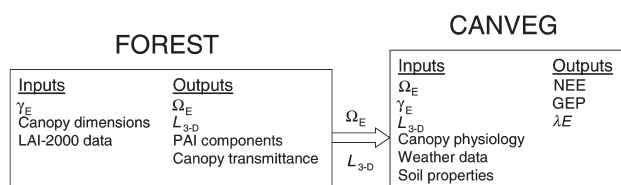
Figure 1. Schematic of FOREST and CANVEG model inputs and outputs, and linkage through FOREST estimates of effective leaf area ( L_{3-D} ) and clumping index at scales larger than shoots ( \Omega_E ). Abbreviations: \gamma_E = needle-to-shoot area ratio for clumping within shoot; \lambda E = ecosystem water vapor exchange; NEE = net ecosystem exchange; and GEP = gross ecosystem productivity.
