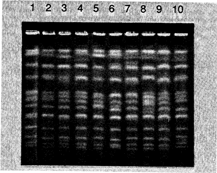
Fig. 1: Electrophoretic karyotypes of Saccharomyces cerevisiae strains. Ethidium bromide stained agarose gel on which the chromosomal DNA molecules of S. cerevisiae have been resolved. Each yeast strain possesses a unique chromosome pattern differentiating it from all other strains: lane 1, 2, 3, 4 = 9, 5, 7, 8 indigenous strains; lane 6, RM1515 SMA inoculated strain; lane 10, S 288 C reference strain. Through the analysis of some samples of the S. cerevisiae colonies isolated during fermentation, it is possible to identify the inoculated strain and to calculate its frequency. The subsequent determination of its hydroxycinnamic acid decarboxylase ability ascertains the stability of the phenotype Pof. — Pulsed field gel electrophoresis was performed through a 1 % agarose gel in 0.5 X TBE (Tris-Borate EDTA) buffer at 14 °C, for 23 h with a switching interval of 60 s for 15 h and 90 s for 8 h, in a CHEF-DR II cell (Bio-Rad Laboratories) apparatus.
