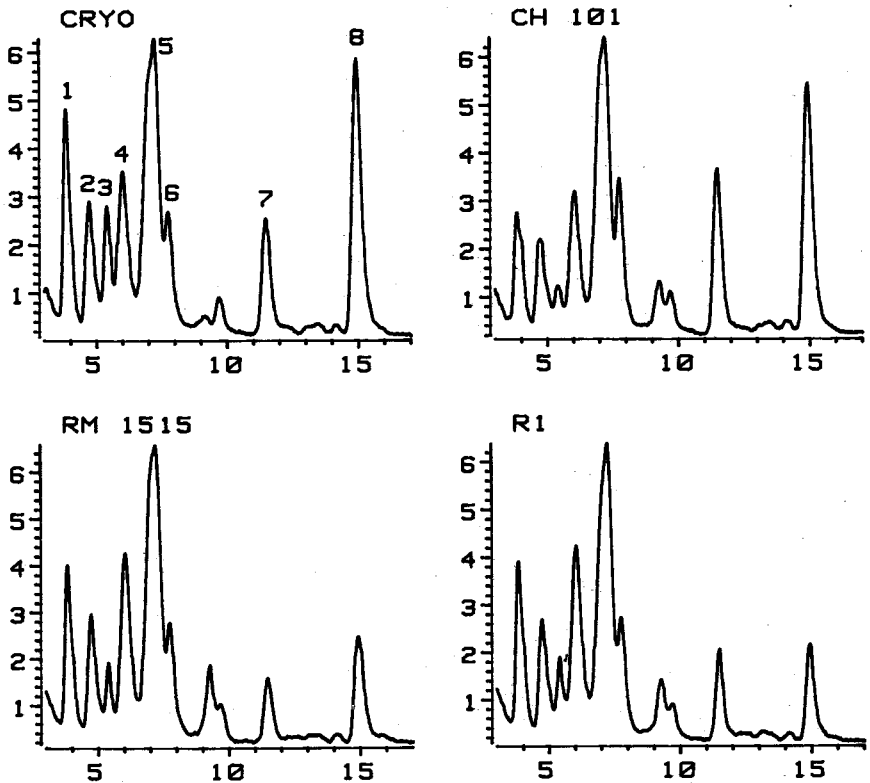
Fig. 2: HPLC analysis of cinnamic compounds in wines from Traminer juice II. 1 = caftaric acid; 2 = p -coutaric acid glucoside; 3 = p -coutaric acid; 4 = 2-S-gluthionyl caftaric acid; 5 = fertaric acid; 6 = caffeic acid; 7 = p -coumaric acid; 8 = ferulic acid.
