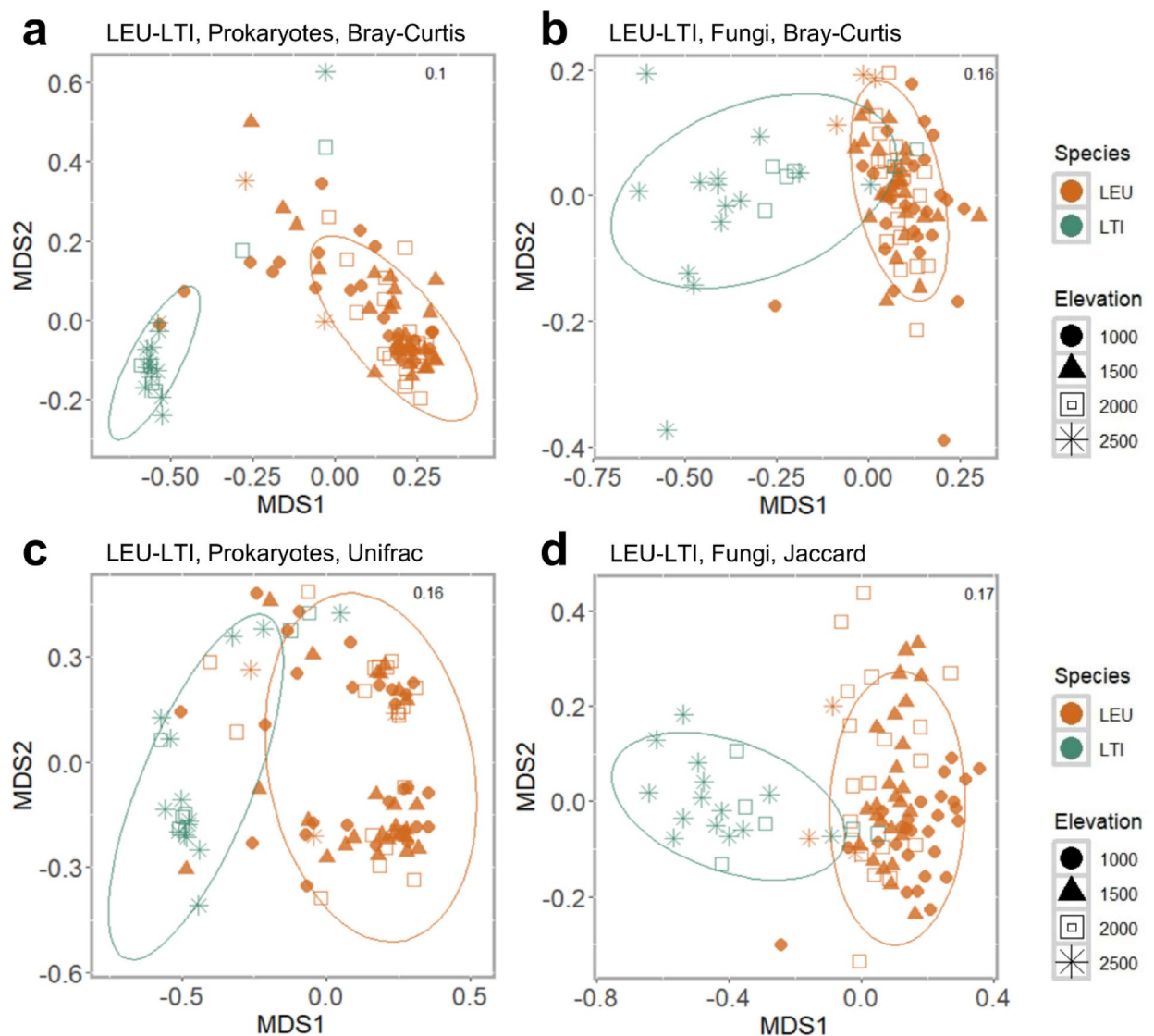
Fig. 4. Non-Metric Multidimensional Scaling (MDS) analyses comparing prokaryote and fungal communities of L. europaeus and L. timidus faecal pellets. Panels (a, c) show prokaryote communities, while (b, d) show fungal communities. Dissimilarities were calculated using Bray–Curtis (a, b), Unifrac (c), and Jaccard (d) indices. Each dot represents a single sample (N = 95). LEU: Lepus europaeus ; LTI: Lepus timidus .
