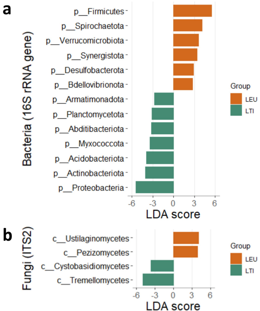
Fig. 3. Differential abundance analysis of prokaryote and fungal communities between the two hare species. (a) Prokaryote phyla and (b) fungal classes with significant differences in relative abundance identified using LEfSE (microeco). The x-axis represents the Linear Discriminant Analysis (LDA) scores, indicating the magnitude of difference between group means. LEU: Lepus europaeus ; LTI: Lepus timidus .
