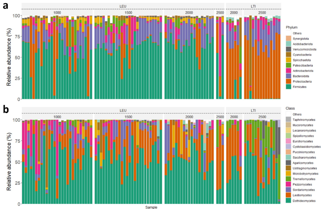
Fig. 2. Relative abundances of faecal prokaryote (16S) and fungal (ITS2) taxa. (a) Phyla based on 16S rRNA gene data and (b) classes based on ITS2 data. Each bar represents a sample, with colors indicating the most abundant taxa as detailed in the legend. Samples are arranged by species (LEU: Lepus europaeus ; LTI: Lepus timidus ) and elevation.
