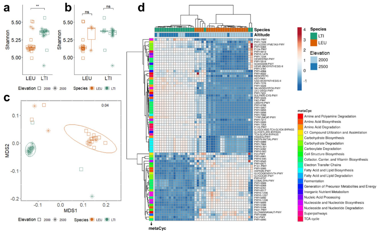
Fig. 6. Functional diversity in Lepus spp. predicted from 16S rRNA gene sequences. (a, b) Shannon diversity of metaCyc pathways in faecal samples from L. europaeus and L. timidus collected at 2000 and 2500 m a.s.l., grouped by species (a) and elevation (b) . Significant differences were assessed using the Wilcoxon rank-sum test. **: p -value \leq 0.01 ; ns: p -value > 0.05 . (c) Non-Metric Multidimensional Scaling (MDS) based on Bray–Curtis dissimilarity estimates of metaCyc pathway abundances; (d) Heatmap of metaCyc pathways showing significant differences in abundance (e.g. \text{Log}_2\text{FC} \geq 1 ; \text{FDR adj. } p\text{-value} \leq 0.01 ) between sympatric L. europaeus and L. timidus across elevations. Rows (i.e. metaCyc pathways; N = 75 ) and columns (i.e. Lepus spp. faecal samples; N = 42 ) are clustered using correlation distance and average linkage. Data are row-centered and scaled to unit variance. Panels (a–c) were created using ggplot2 43 (a, c) and ClustVis 49 (d) and formatted using GIMP v2.10.18 (The GIMP Development Team, 2019). LEU: Lepus europaeus ; LTI: Lepus timidus .
