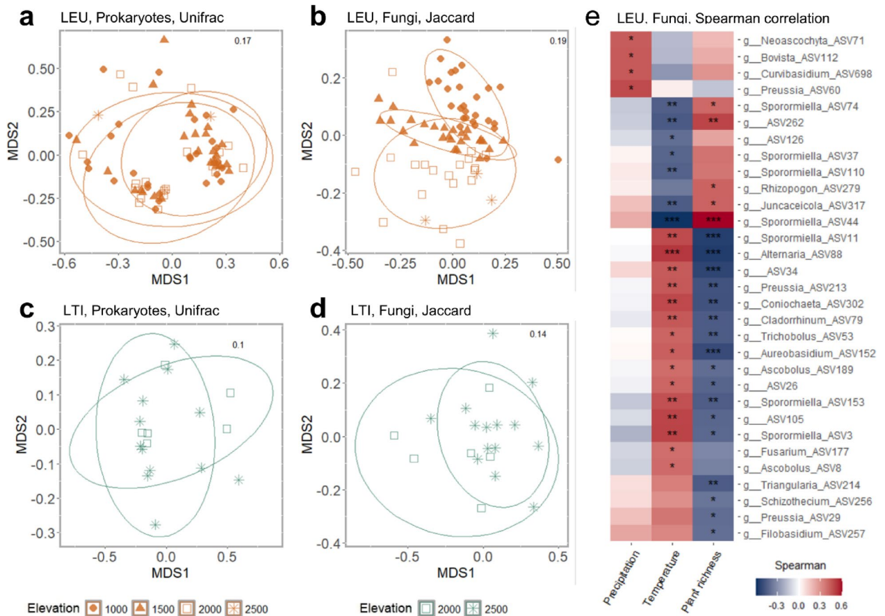
Fig. 5. Non-Metric Multidimensional Scaling (MDS) and Spearman correlation analyses comparing prokaryote and fungal community structures across different elevations. (a, b) MDS clustering of prokaryote and fungal communities in L. europaeus faecal samples; (c, d) MDS clustering prokaryote and fungal communities in L. timidus faecal samples. Each symbol represents a single faecal sample, with different shapes indicating elevation; (e) Spearman correlation analysis between environmental variables (x-axis) and L. europaeus faecal fungal ASVs (y-axis). Correlation coefficients indicate the strength and direction of the relationships. Significant correlations are indicated (* p -value < 0.05; ** p -value < 0.005; *** p -value < 0.0005). LEU: Lepus europaeus ; LTI: Lepus timidus .
