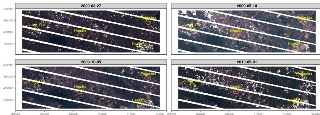
Figure 7. RGB composite of the four image-sets used for Land Surface Temperature estimation, with both SCL-off and cloud cover assessment masks. Images are around 12 km in width.
