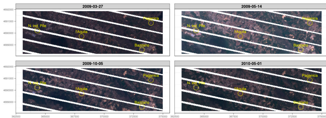
Figure 6. RGB composite of the four image-sets used for Land Surface Temperature estimation (Scan Line corrector (SCL)-off mask applied, no cloud cover assessment); images are around 12 km in width.
