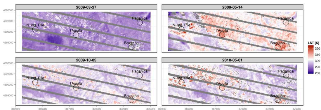
Figure 8. Land Surface Temperature Maps (LST) without rescale. The gray pixels correspond to the SCL-off and cloud cover assessment masks. Images are around 12 km in width.
