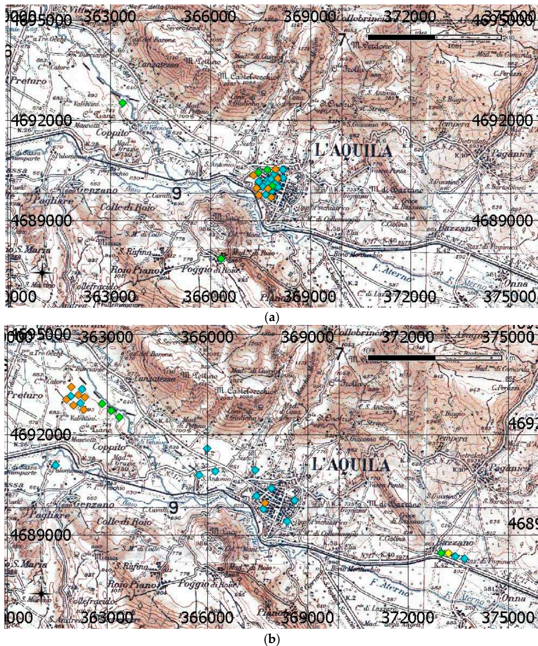
Figure 2. L'Aquila, before (a) and after (b) the main seismic event: Overlapped grid is Universal Transverse Mercator Projection (UTM) WGS84/ETRF00. Scale bar (upper right) is 4 km, and the north-pointing arrow (lower left) indicates the geographic north.
