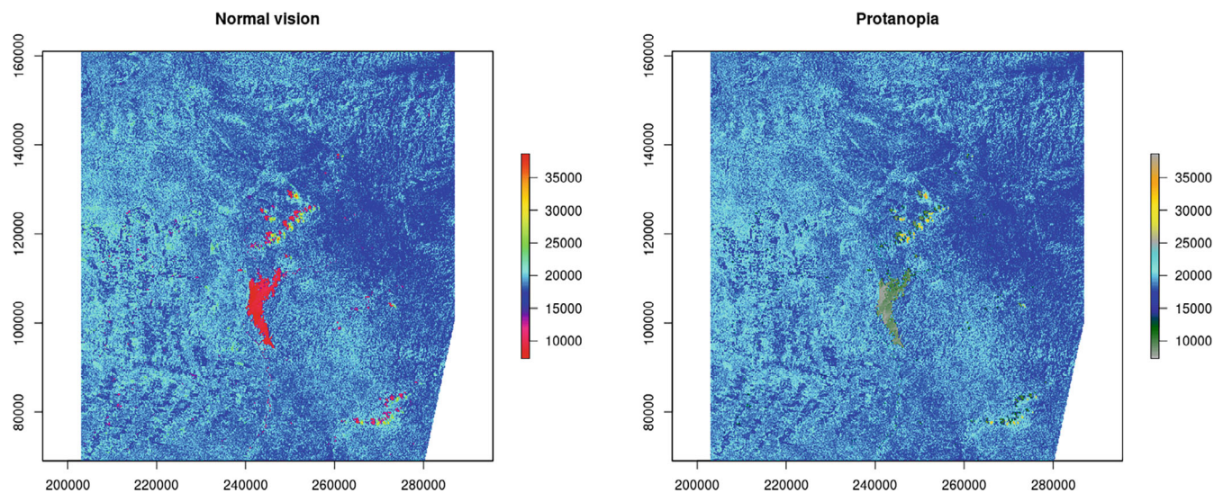
FIGURE 2 The Amazon forest between Boa Vista and Caracarai (Brazil), band 8 of a Sentinel-2 image (near infrared) plotted with a rainbow color palette (left). A simulation of the vision with protanopia or deuteranopia is provided on the right image. It shows the blurring effect that can occur with colorblindness.
