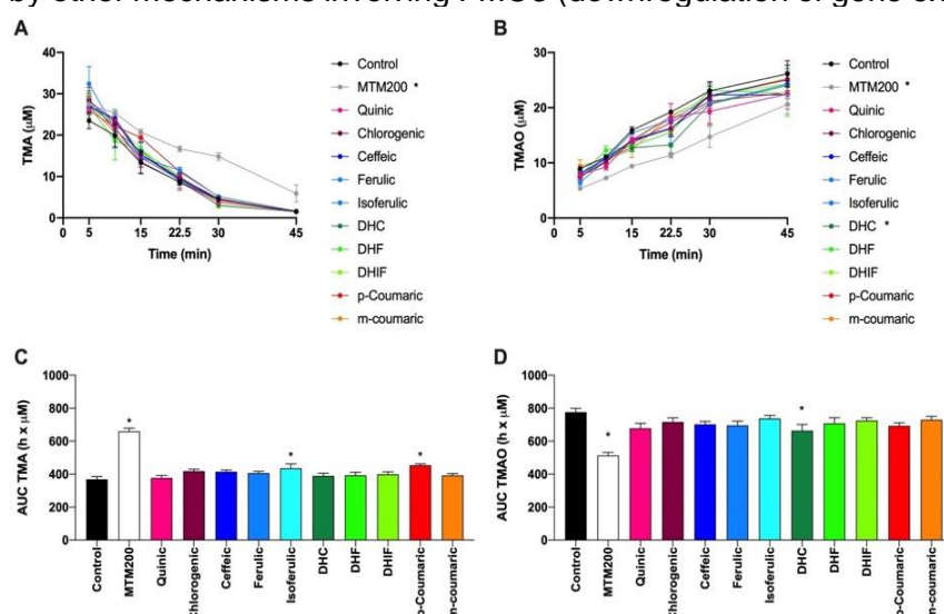
Figure 1: Effect of chlorogenic acid-related compounds on kinetics of TMA (A) and TMAO (B), and areas under the curve of TMA (C) and TMAO (D). *different vs. control by Two-Way (A&B, factors: time, treatment) and by One-Way (C&D) ANOVA (Dunnett's post hoc test, p < 0.05 ).
