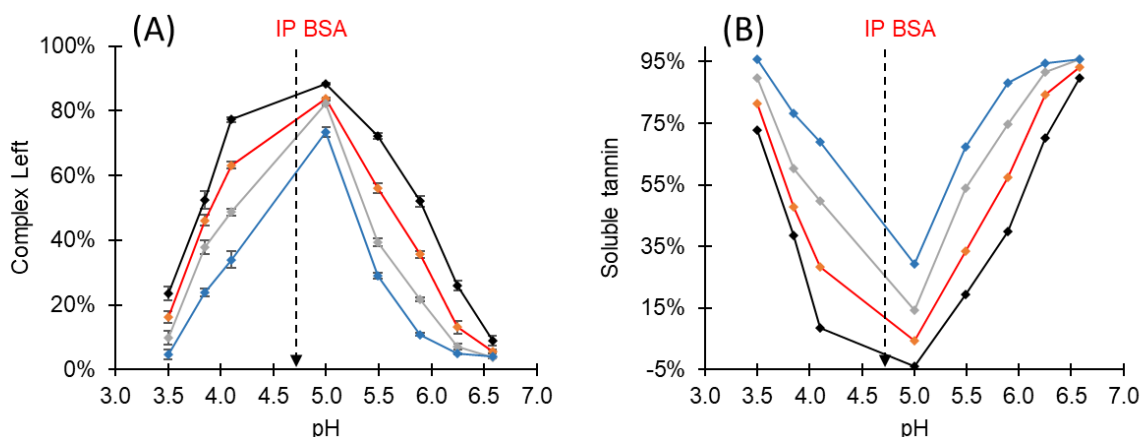
Figure 1 : The amount of HT-BSA complex left (A) and the amount of soluble tannin after pH adjustment of the reaction solution. The PGG:BSA ratios in the initial complexation reaction at pH 5 were 5 :1 (black line), 4 :1 (orange line), 3 :1 (grey line) and 2 :1 (blue line).
