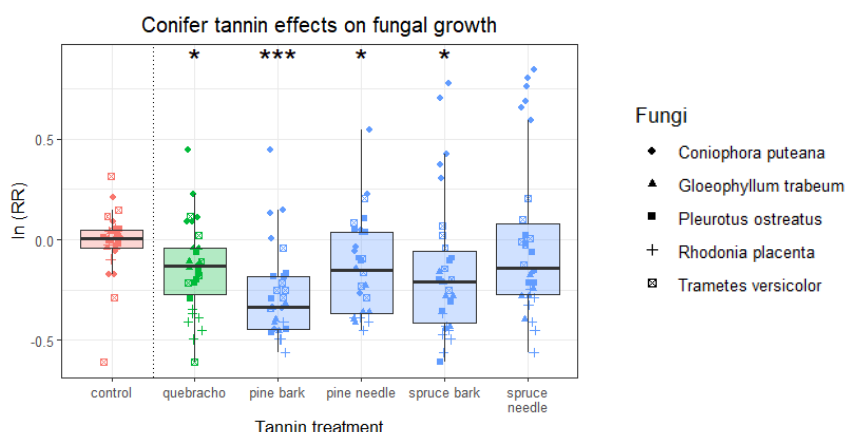
Figure 1: Bioactivity of studied tannin fractions against five fungal saprotrophs, shown as log-response ratio (ln(RR)) of growth relative to the control treatment (* 0.01<p<0.05, *** p<0.001)
