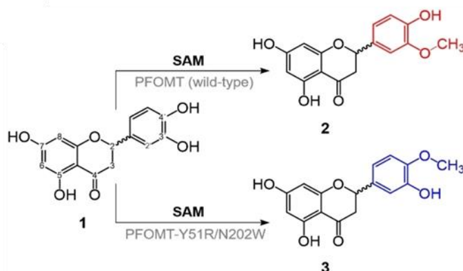
Figure 1 : Regiospecific attachment of a methyl group to the flavanone eriodictyol (1) yields homoeriodictyol (2) with a vanilloid B-ring motif (red), or hesperetin (3) with an isovanilloid motif B-ring (blue).
