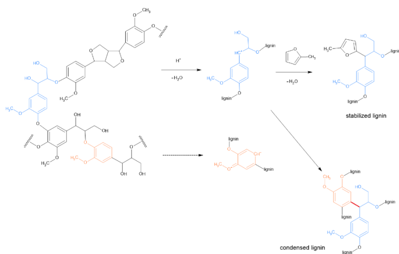
Figure 1: Scheme of condensation and substitution reactions
