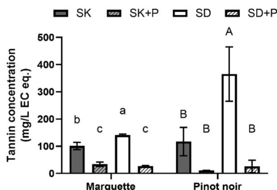
Figure 3. Tannin concentration (mg/L) in supernatants of skin (SK), skin with flesh (SK+P), seed (SD), and seed with flesh (SD+P) after five days of soaking in a wine-like solution. Lowercase and uppercase letters indicate a significant difference ( p < 0.05 ) among treatments when compared in Marquette and Pinot noir tissues, respectively.
