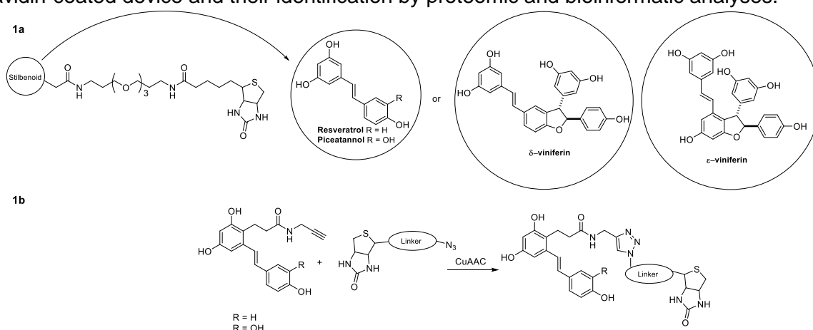
Figure 1: structures of the proposed stilbenoid-bearing probes
