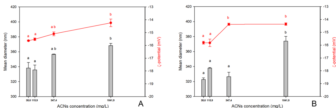
Figure 6 - Effect of ACNs concentration on the mean diameter and \zeta -potential of coacervates on day 0 (A) and day 14 (B). Different lowercase letters indicate significant differences ( p < 0.05 ) between samples. Each data is expressed as mean of triplicates \pm standard error.
