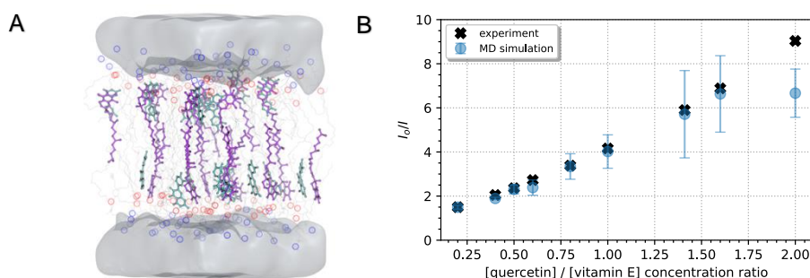
Figure: (A) Simulated noncovalent association (quercetin:vitaminE) in a lipid bilayer membrane, (B) Quenching Stern-Volmer plot
