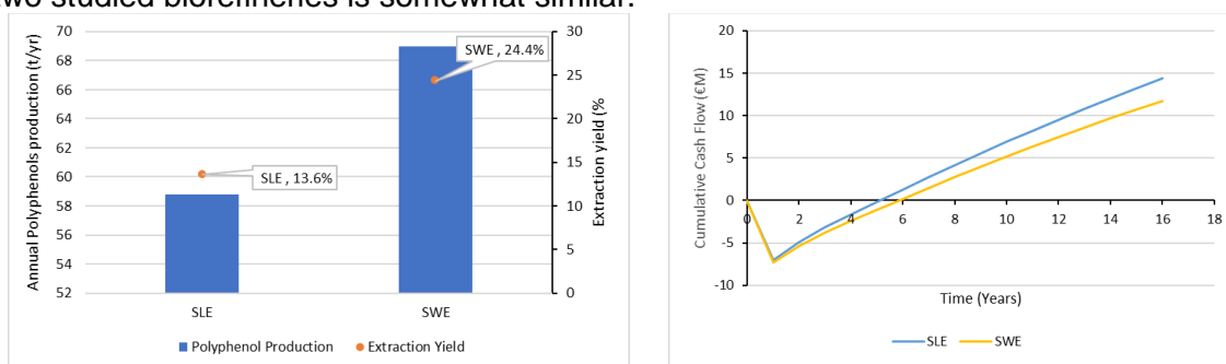
Figure 1. Technical performance (left) and cumulative cash flow (right) comparison for SLE and SWE processes.
