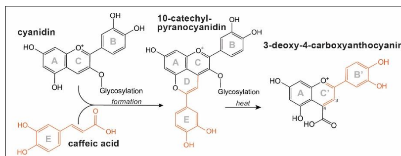
Figure 1: Formation of 10-catechyl-pyranoanthocyanins and the 3-deoxy-4-carboxyanthocyanin elucidated in this experiment. Rings B' and C' correspond to rings E and D of the precursor compound, respectively.
