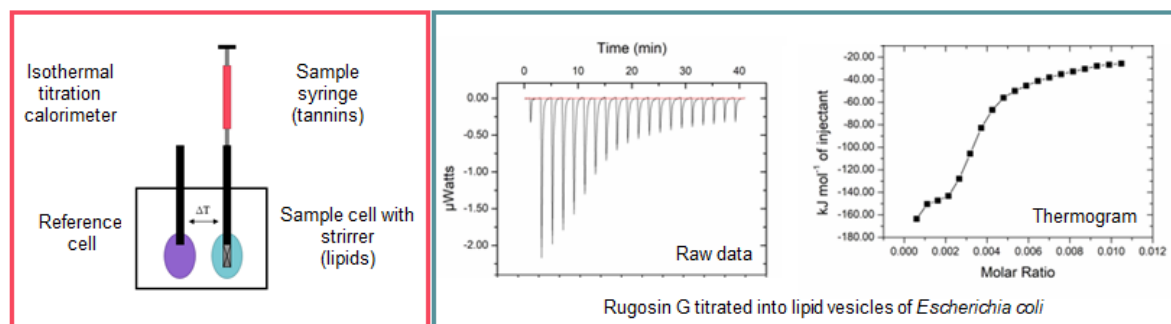
Figure 1: Ellagitannin rugosin G titrated into lipid vesicles by isothermal titration calorimetry
