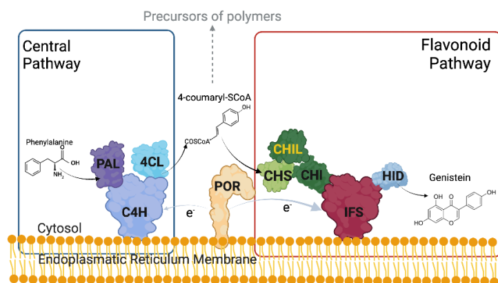
Figure 4. Schematic representation of the phenylpropanoid pathway and the proteins involved in the genistein biosynthesis.
