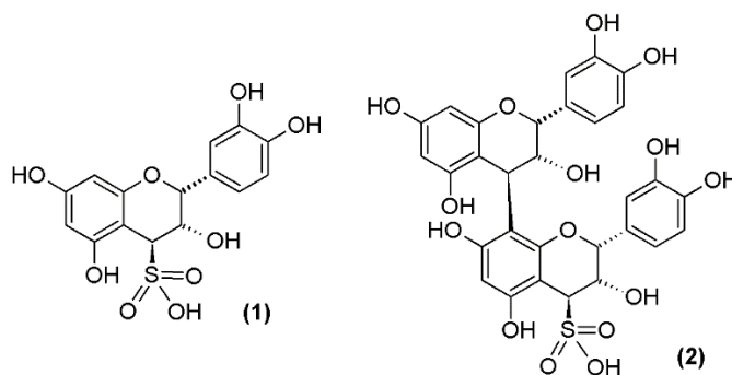
Figure 1 : The structure of epicatechin-4 \beta -sulfonate (1) and 4 \beta -sulfoprocyanidin B2 (2)
