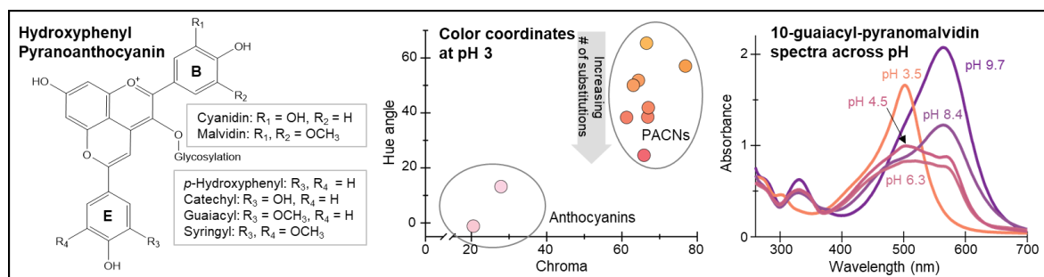
Figure 1 : Chemical structure of the 8 pyranoanthocyanins (PACNs) evaluated, effect of number of B and E ring substitutions on color of PACN, and spectral changes across pH for 10-guaiacyl-pyranomalvidin-3-glucoside. Color of circles and spectra represent the solution color.
