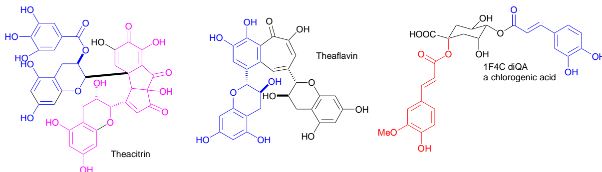
Figure 1 : Selected polyphenol structures from black tea and coffee
