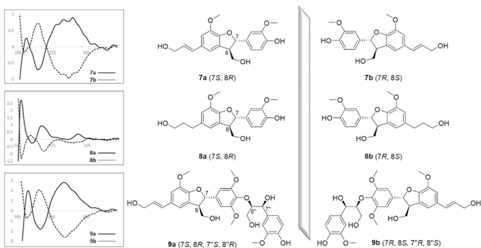
Figure 1 : Experimental ECD spectra of 7a/7b , 8a/8b , and 9a/9b
