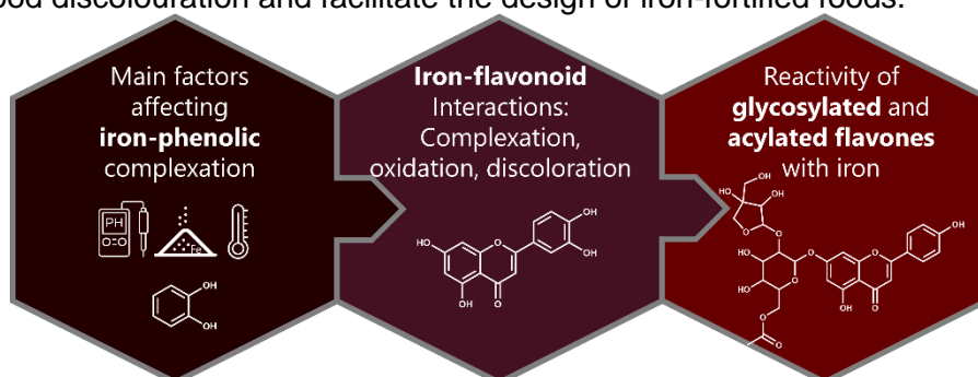
Figure 1: Unravelling discolouration due to iron-phenolic interactions
