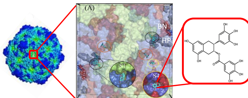
Figure 1: Docking sites identified for EGCG around the 2-fold axes of symmetry of Coxsackievirus A9 (docking performed by O. Sheik Amamuddy and Özlem Tastan Bishop (Rhodes University, SA))
