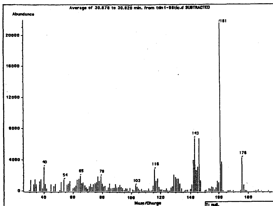
Fig. 4: MS spectrum of TDN- d_4 .
