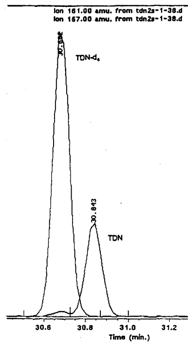
Fig. 3: Part of a GC-SIM/MS profile with TDN ( m/z=157 ) and TDN- d_4 ( m/z=161 ) peaks.
